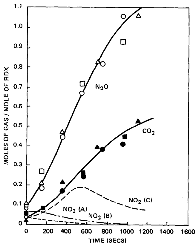
Fig 10 Concentration-time profiles of N_2O , CO_2 , and NO_2 for three reactor volumes. N_2O and CO_2 curves: o and •, 26ml; \Delta and \blacktriangle , 100ml; \square and \blacksquare , 300ml. NO_2 curves: A, 26ml; B, 100ml; C, 300ml. Initial weight of RDX, 40mg. (See Fig 11 for data points of NO_2 )
